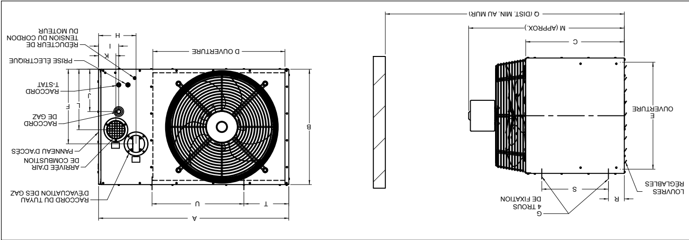
Figure 24.1 - Plans cotés
