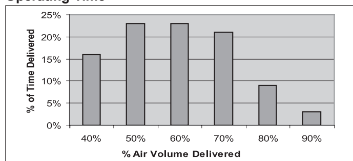
Figure 13.1 - Typical Air Volume Delivery vs. Operating Time
