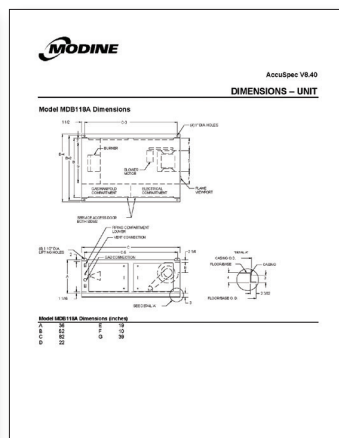
Dimensional Drawings
