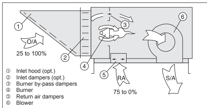
Figure 4.2 - Return Air Unit (MRB)
