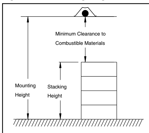
Figure 10.2 - Stacking Height
