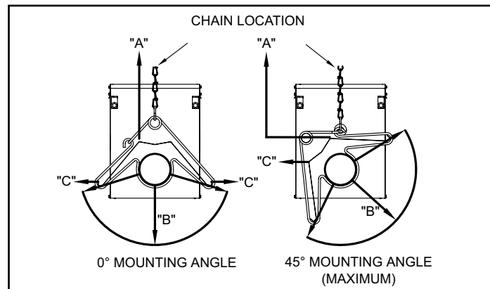
Figure 10.1 - Combustible Material Clearances - Straight Tube
