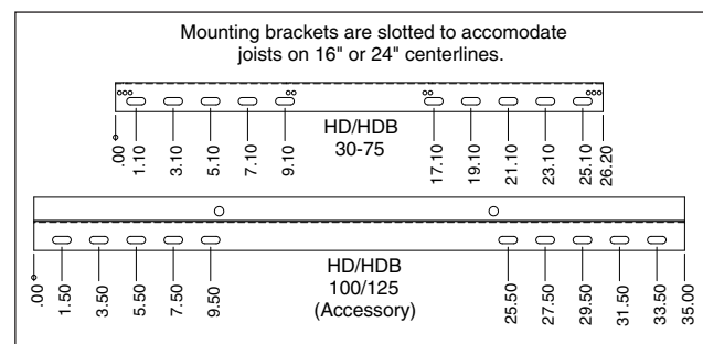
Figure 19.3 - Mounting
