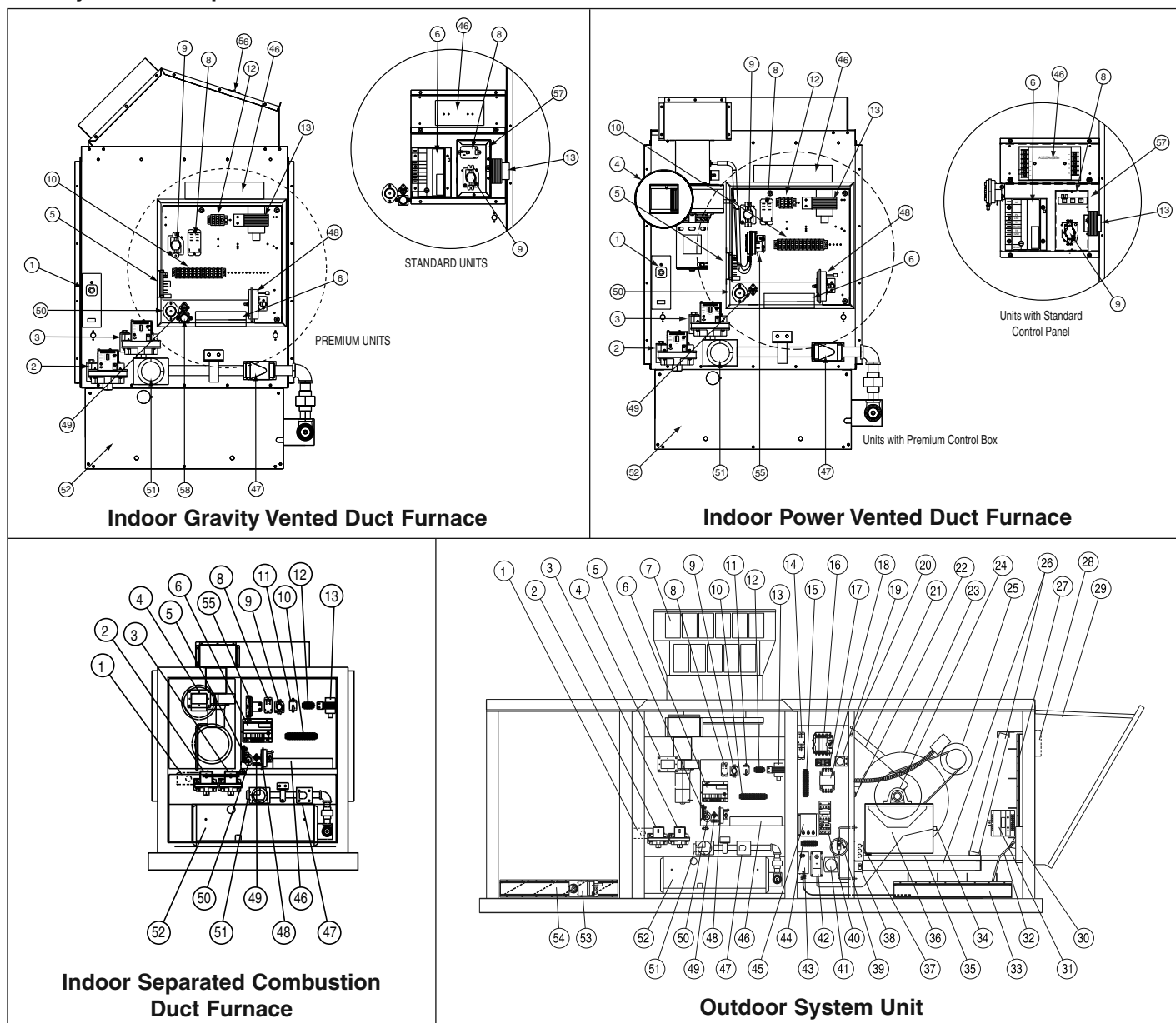
Figure 24.1 Factory Mounted Option Locations
