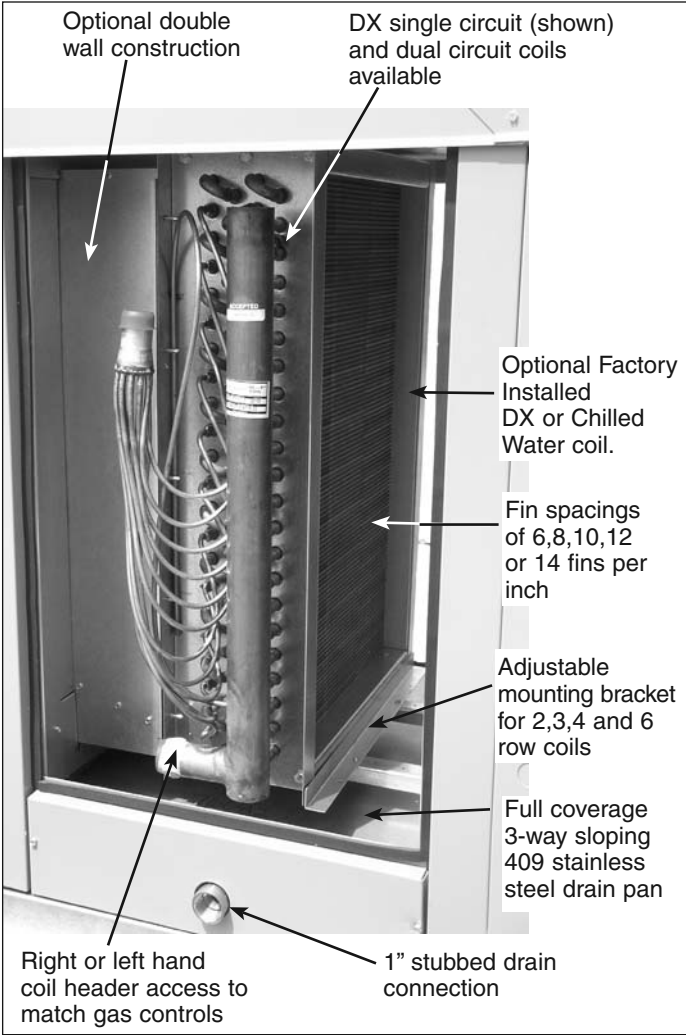
Figure 62.1 Cooling Section
