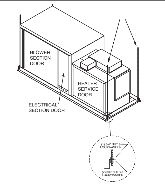
Figure 4.1 - Unit Suspension Method
