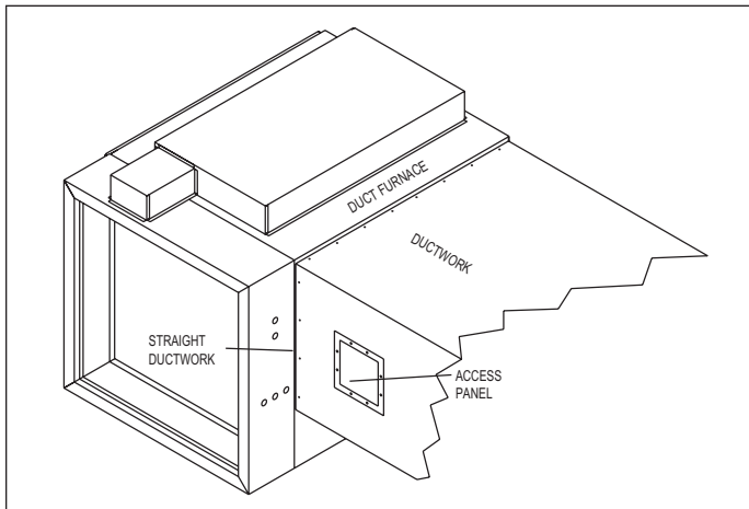
Figure 5.1 - Furnace Discharge Duct Connection
