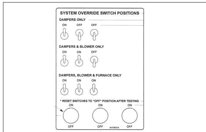
Figure 29.4 - Service Switches
