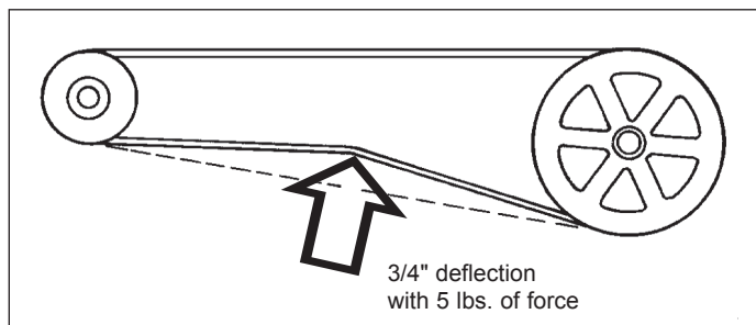
Figure 20.2 - Belt Tension Adjustment
