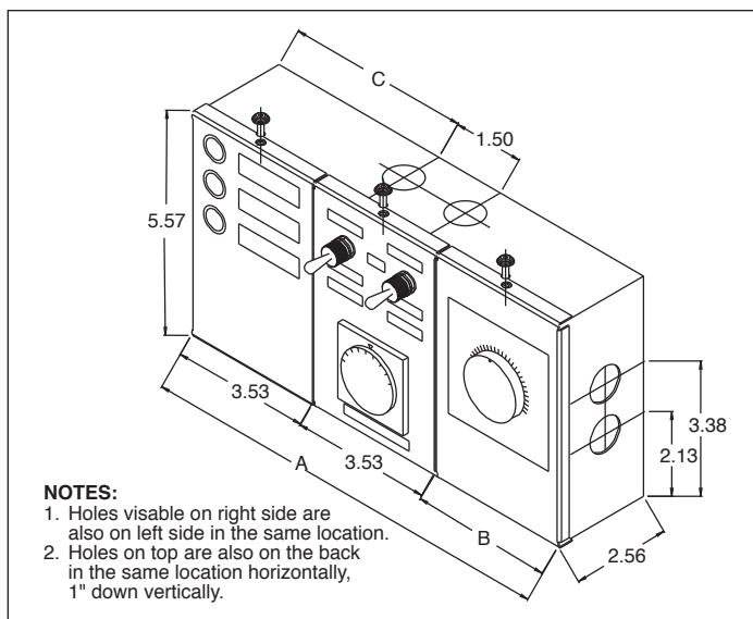
Figure 46.1 - Remote Panel Dimensions
