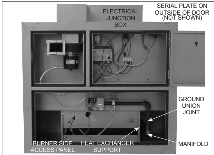
Figure 48.1 - Manifold Assembly Removal
