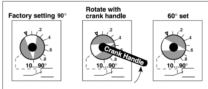
Figure 27.1 - Adjusting the Damper End Switch
