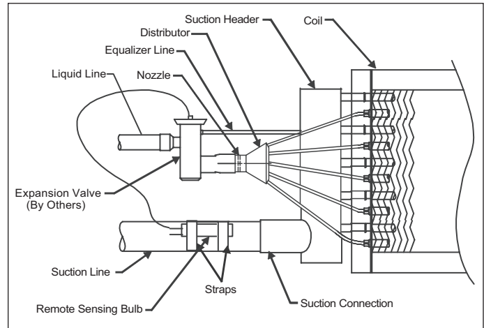
Figure 16.2 - General DX Piping
