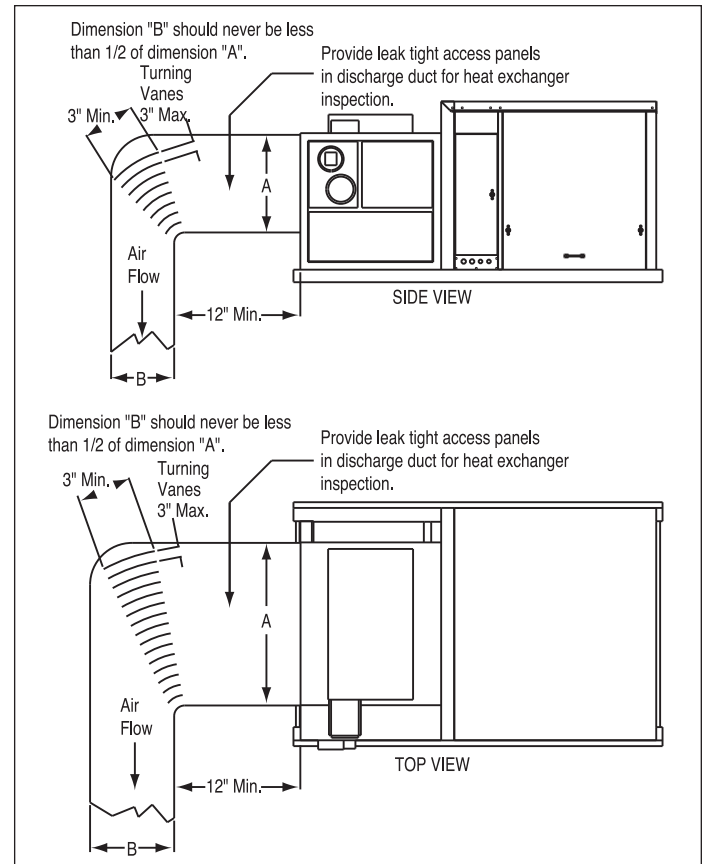
Figure 5.3 - Recommended Field Installed Discharge Duct Configurations for Blower Package Units
