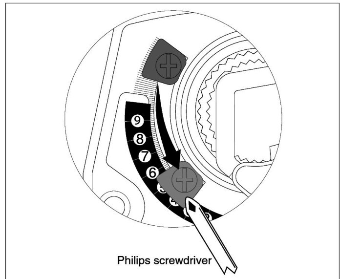
Figure 26.2 - Two-position Damper Actuator and Limiter
