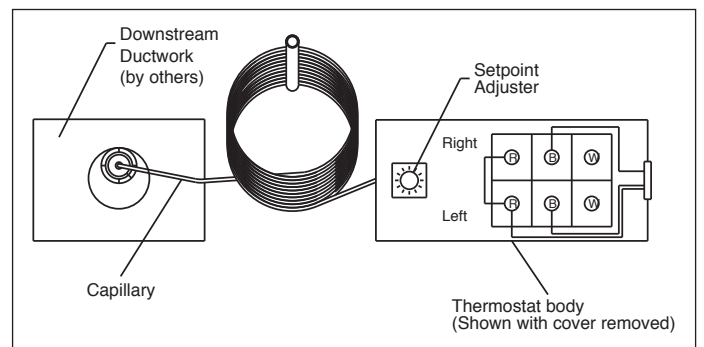
Figure 23.2 - Two-Stage Capillary Type Thermostat
