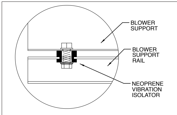
Figure 28.1 - Blower/Motor Vibration Isolation
