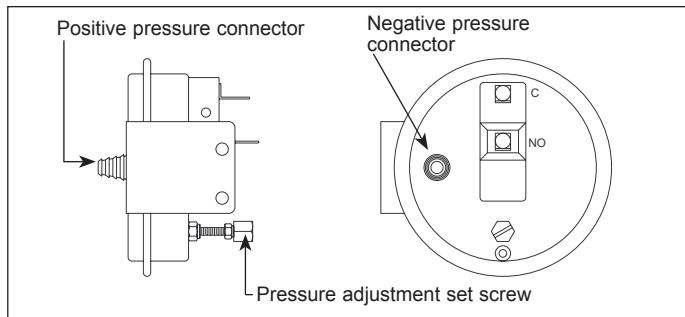
Figure 29.1 - Dirty Filter Pressure Switch and Air Flow Proving Switch
