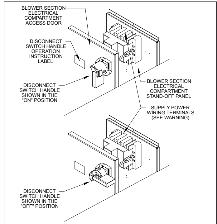
Figure 25.1 - Dead Front Disconnect Switch Assembly
