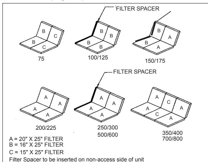
Figure 47.1 - Filter Replacement Arrangement for Blower Size (Digit 16) A, B, C, D, E, F, G and H
