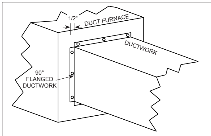
Figure 5.2 - Blower Section Inlet and Cooling Coil Section Discharge Duct Connections
