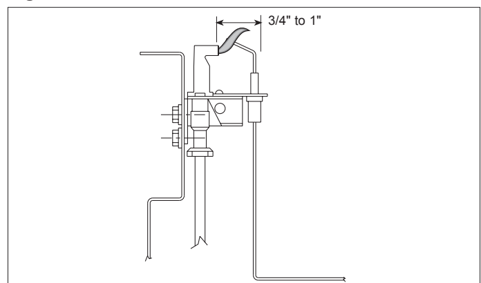
Figure 18.1 - Correct Pilot Flame
