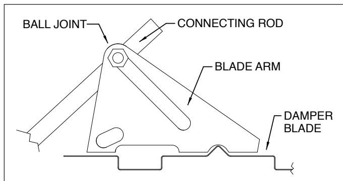
Figure 20.3 - Damper Linkage Adjustment
