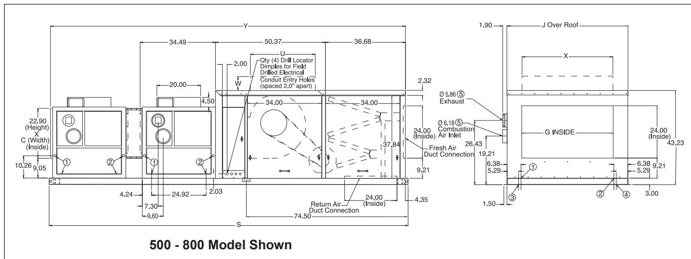
Figure 43.2 - DCS Separated Combustion Cooling Package Unit Dimensions with Blower Type I, J, or K
