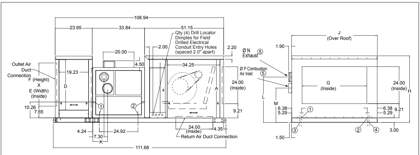
Figure 42.2 - DCS Separated Combustion Cooling Package Unit Dimensions
