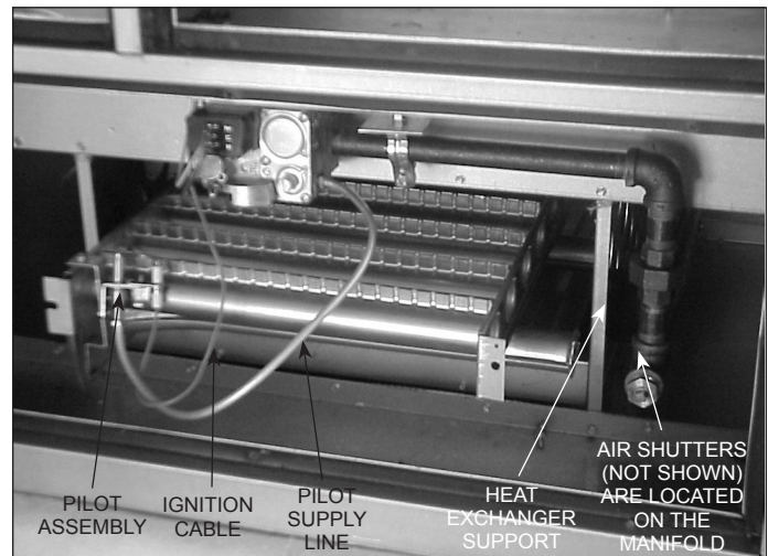
Figure 48.2 - Burner and Pilot Assembly Removal
