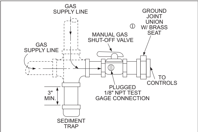
Figure 12.1 - Recommended Sediment Trap/Manual Shut-off Valve Installation - Side or Bottom Gas Connection
