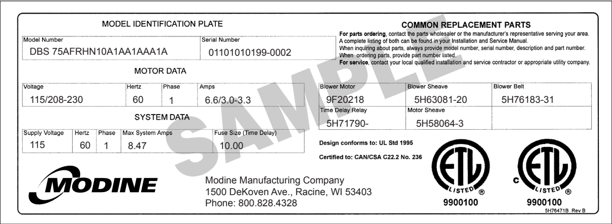
Figure 52.1 - Model Identification Plate
