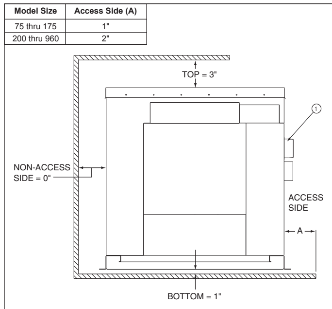
Figure 3.1 - Combustible Material Clearances
