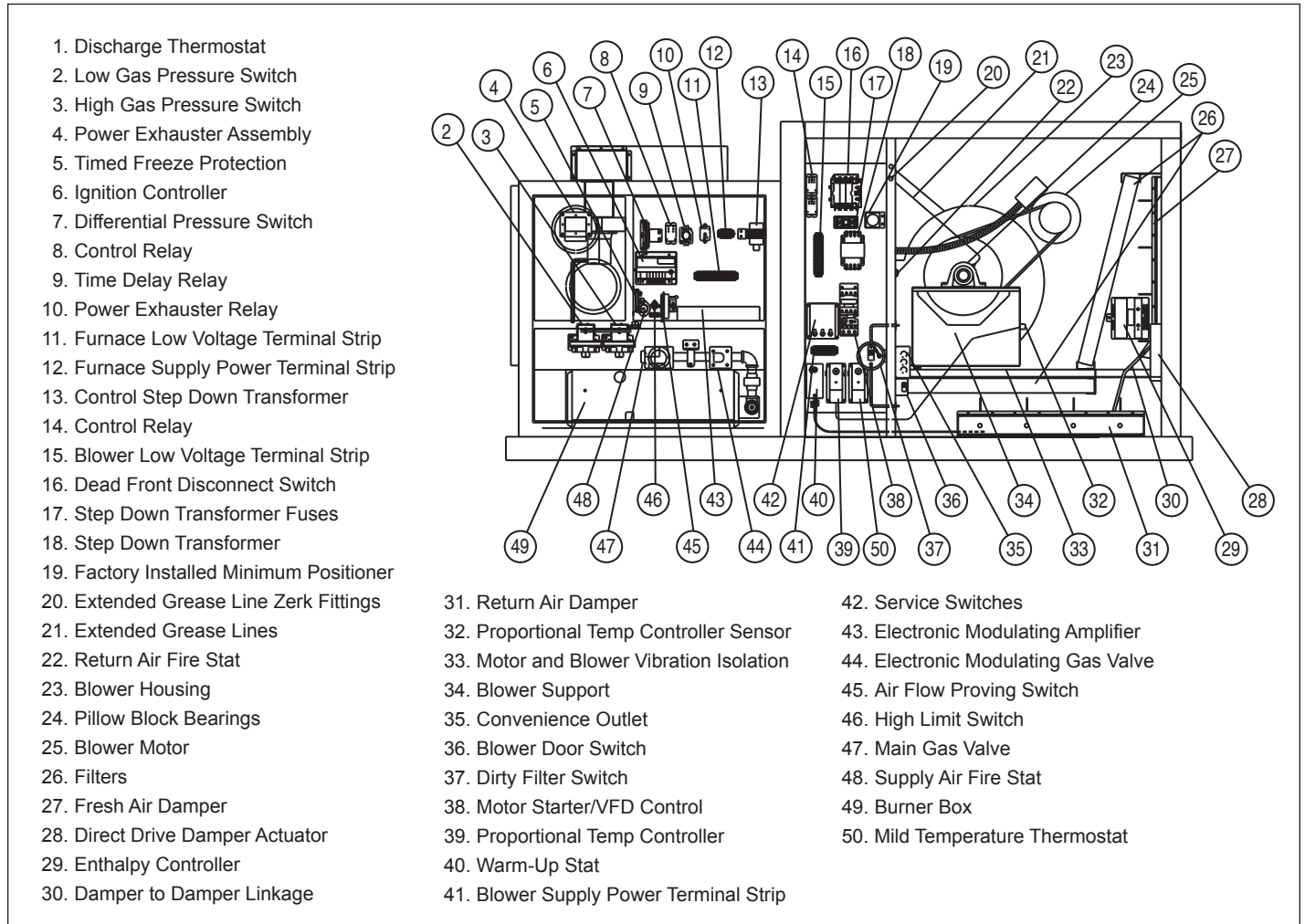
Figure 23.1 - Factory Mounted Option Locations
