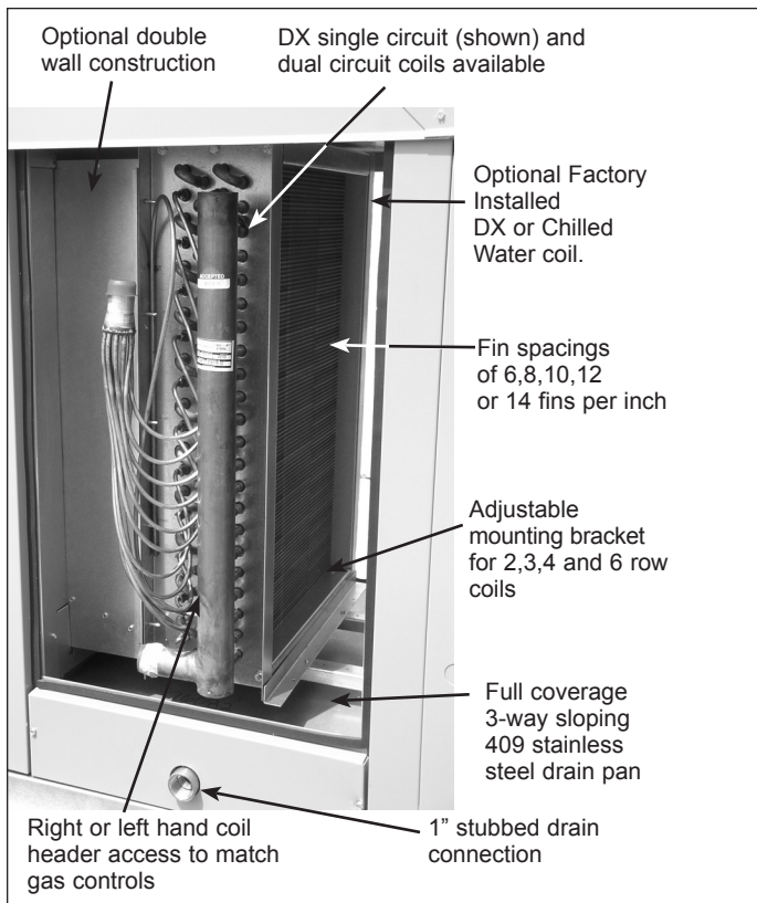
Figure 16.1 - Cooling Section
