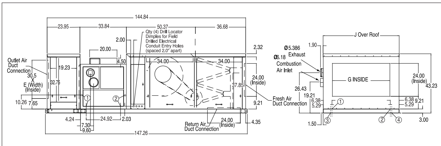
Figure 43.2 - DCS Separated Combustion Cooling Package Unit Dimensions with Blower Type I, J, or K
