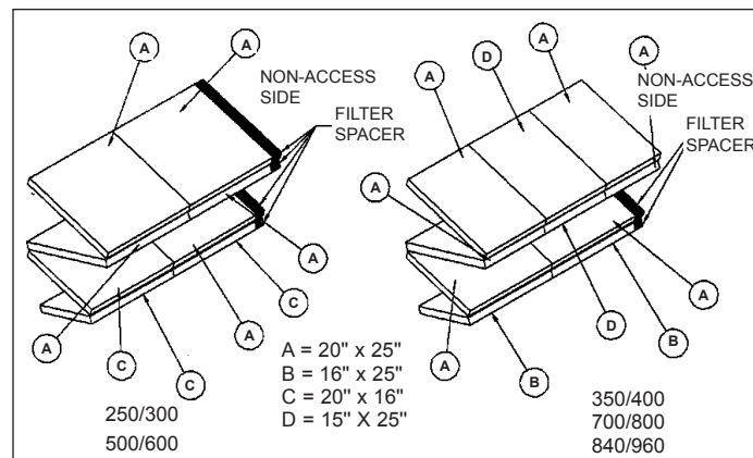
Figure 47.2 - Filter Replacement Arrangement for Blower Size (Digit 16) I, J, K, and L
