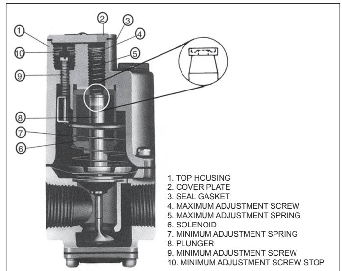
Figure 19.2 - Maxitrol Modulating Valve Adjustments
