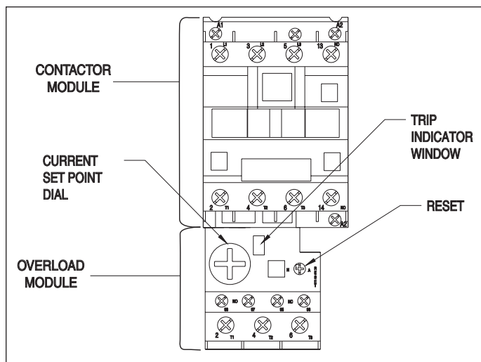
Figure 29.2 - Motor Starter
