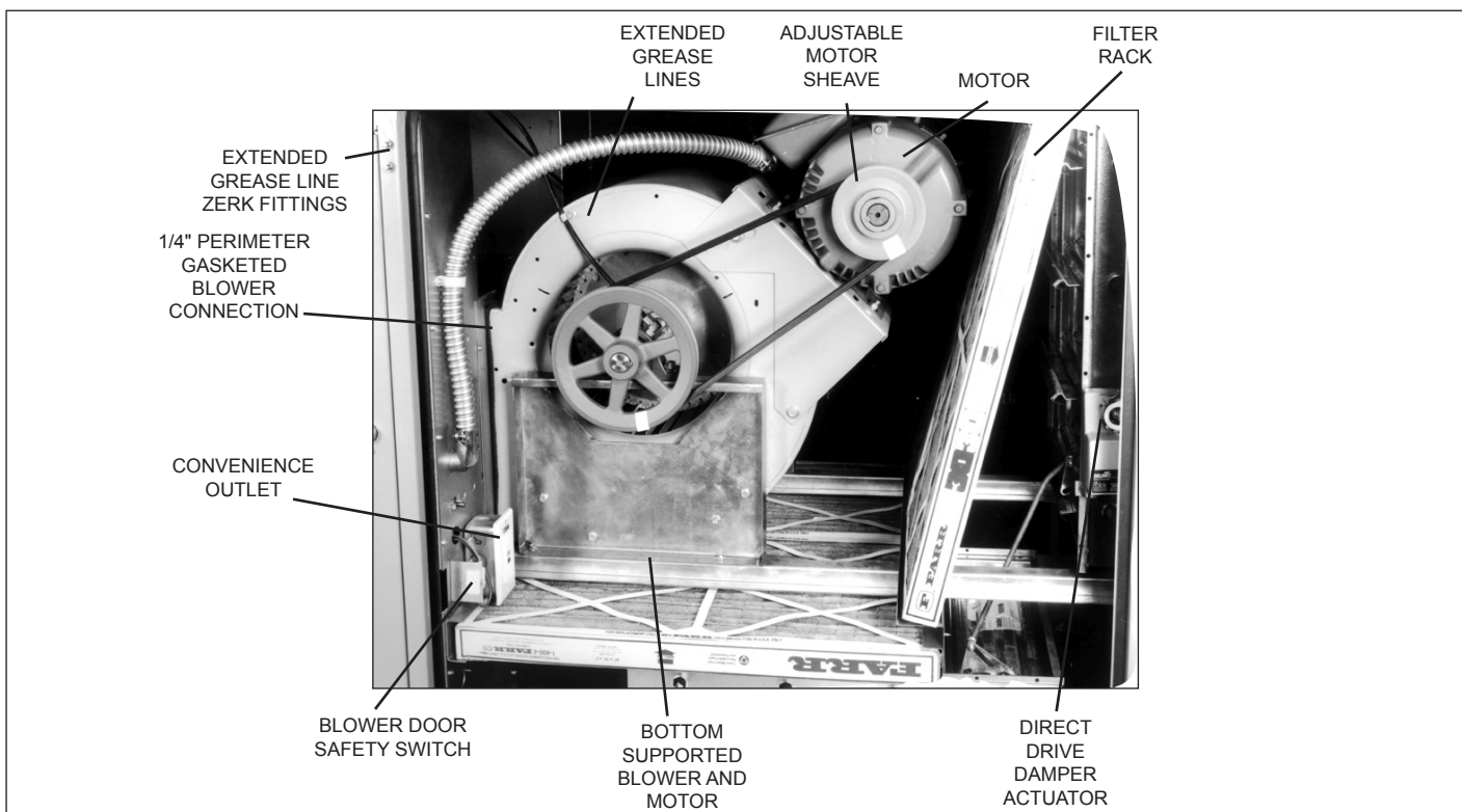
Figure 37.1 - Blower Section
