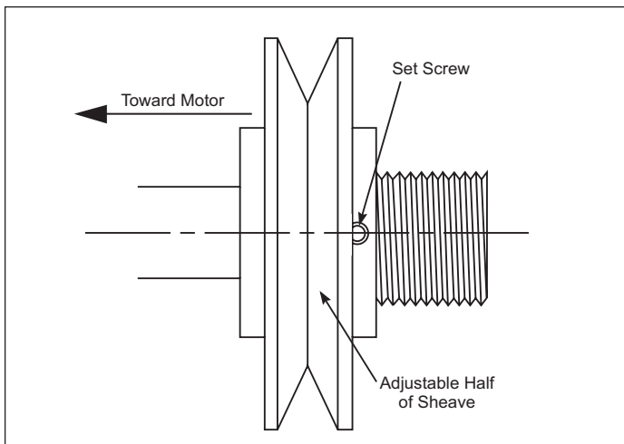
Figure 20.1 - Motor Sheave Adjustment
