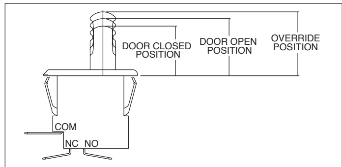
Figure 28.2 - Blower Door Switch with Manual Override
