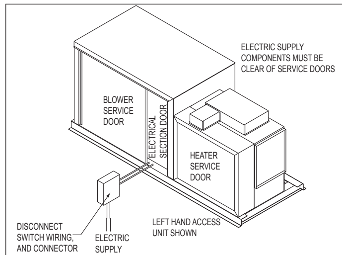
Figure 15.1 - Recommended Accessory Field Installed Disconnect Switch Mounting Locations
