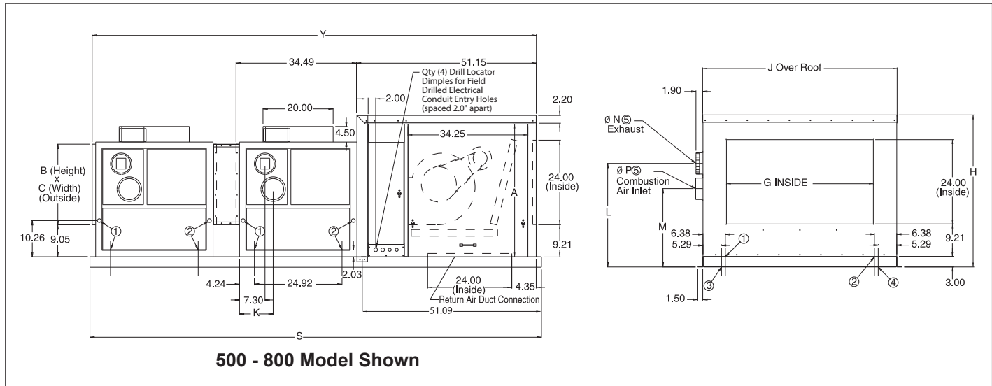
Figure 42.1 - DBS Separated Combustion Blower Package Unit Dimensions
